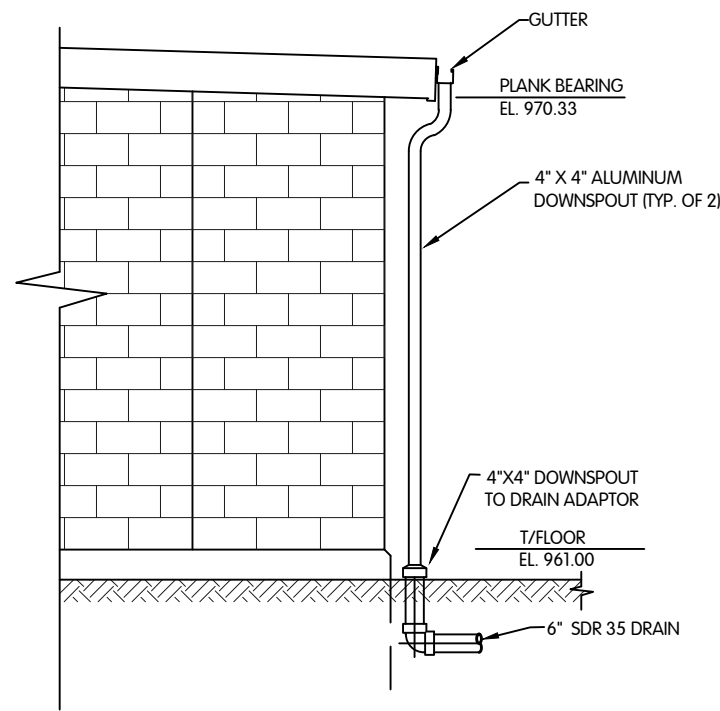
GUTTER AND DOWNSPOUTS NTS
