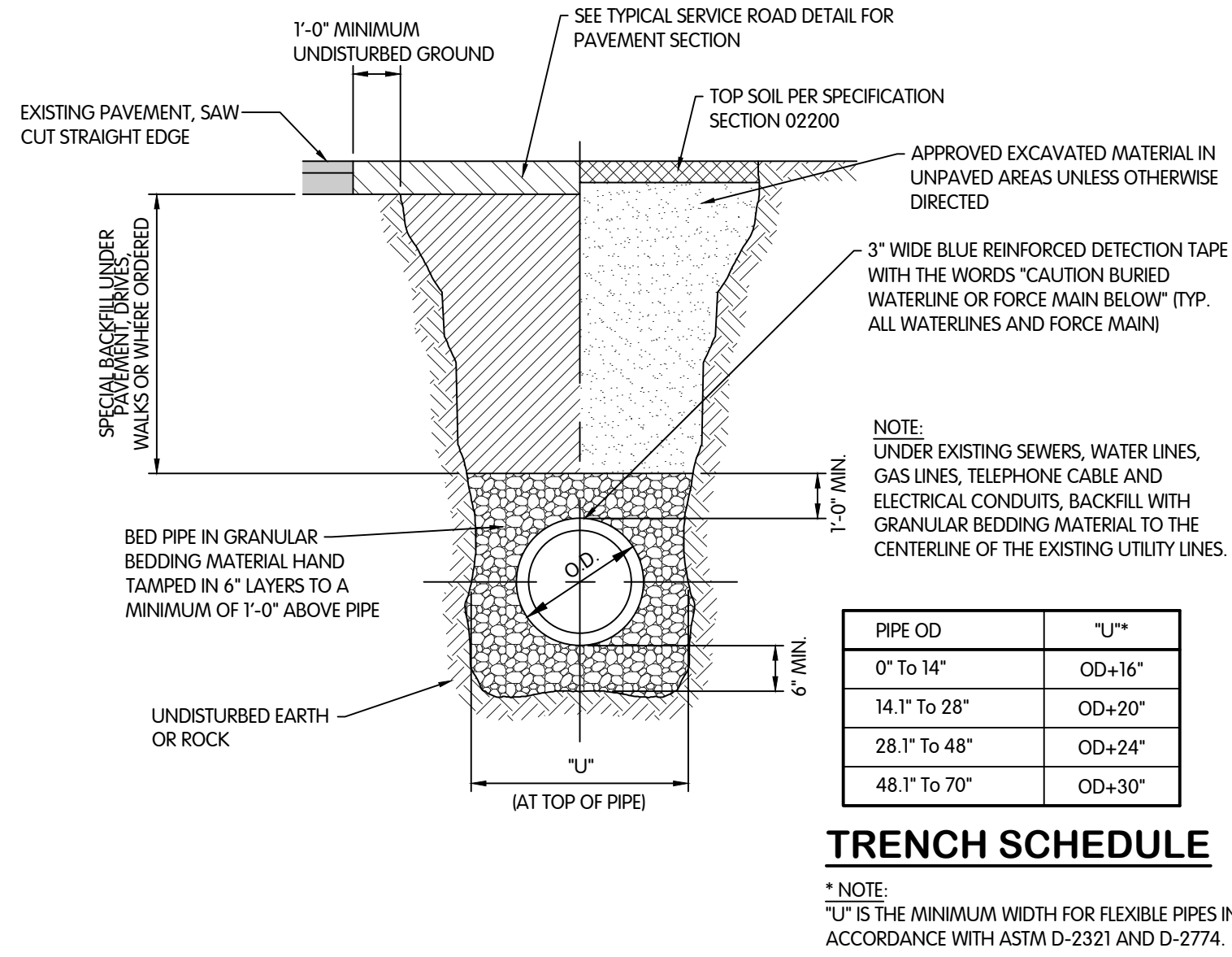
TRENCH DETAIL FOR FLEXIBLE PIPE NTS
